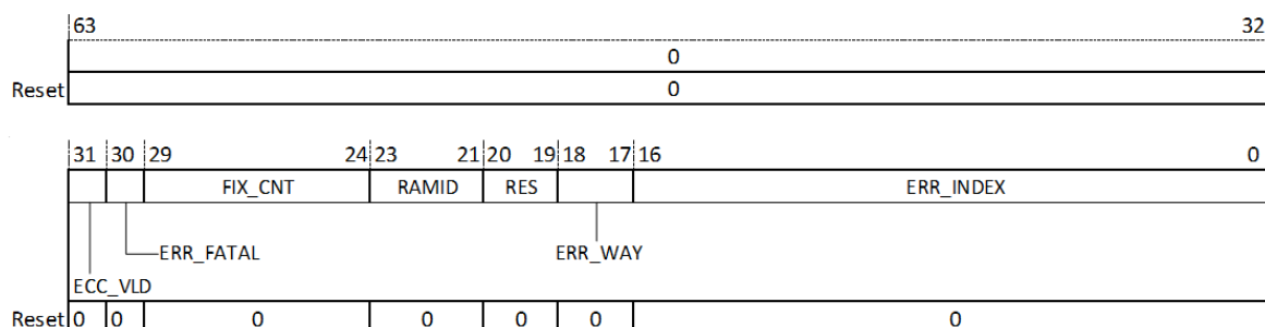
图 18.16: L1Cache ECC 寄存器 (MCER)
